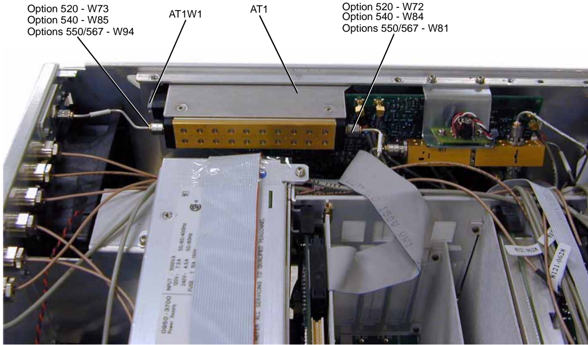
Figure 3 Option 1E1 (Rear Panel RF Output)
